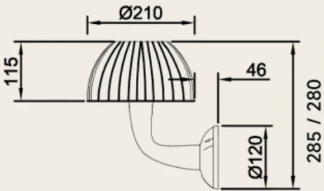
LV VERSION(DC12W)
