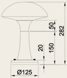
LV VERSION(DC12W)
