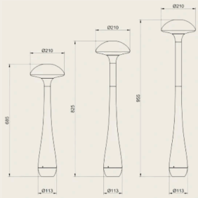
LV VERSION(DC12W)
