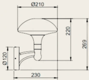
LV VERSION(DC12W)
