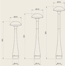
LV VERSION(DC12W)
